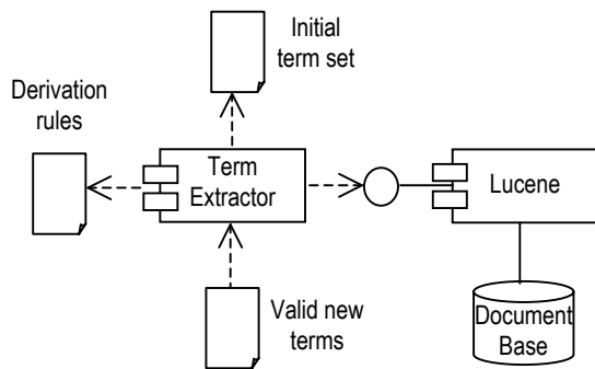
Figure 3. UML diagram of the components involved in the extraction and validation process
