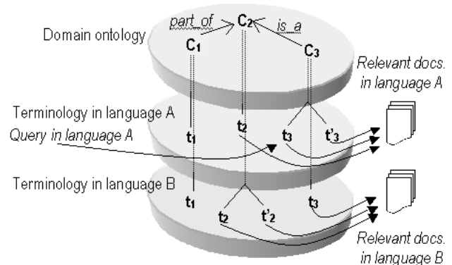
Figure 1. CLIR using a domain ontology
